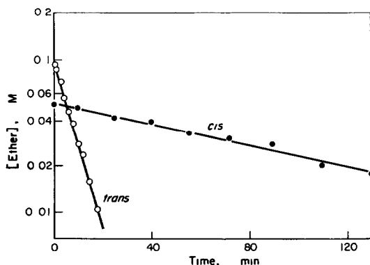
Fig 1. First-order plots for the hydrolysis of 1c (●) and 1t (○); [HCl] = 0.2 M in 80% aqueous dioxane, 25°C.
